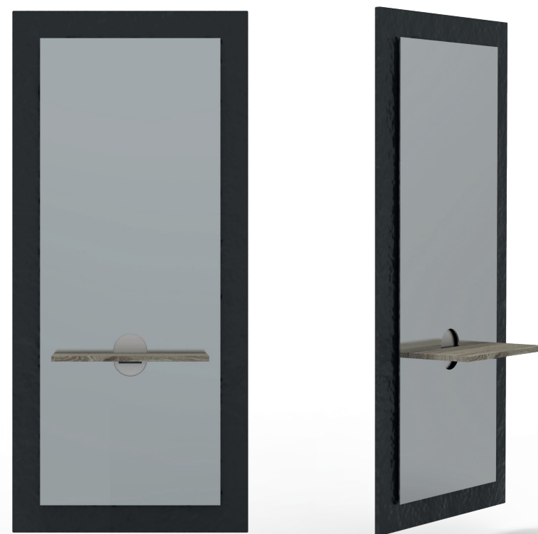
Betula | Frontpanel: Dimensions 1860 x 840 mm anthracite artificial leather. Worktop: Dim. 540 x 250 mm in light oak laminate Mirror: Dim. 1660 x 640 mm with cutout for worktop.
